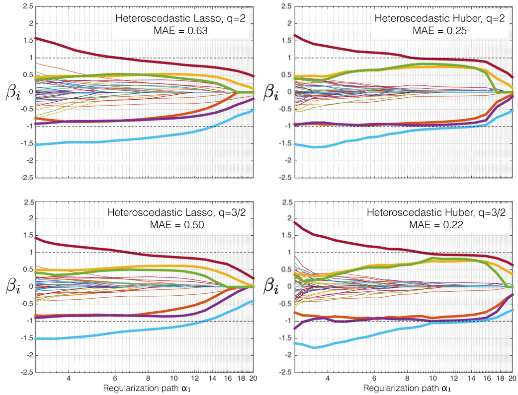
Figure 4: Generalized heteroscedastic lasso and Huber solutions for \bar{b} when q = 2 (top panel) and q = 3/2 (bottom panel) across the relevant \alpha_1 -path. The minimally achievable mean absolute error (MAE) is shown for all models. The six highlighted \beta_i trajectories mark the true non-zeros entries of \bar{b} . The dashed black lines show the values of the true \bar{b} entries.
