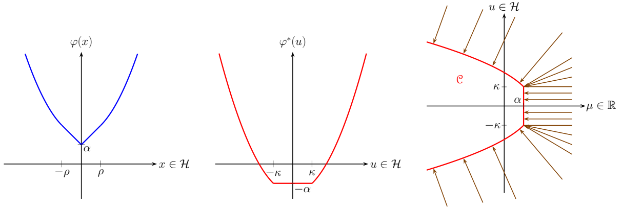
Figure 1: Geometry of the computation of \text{prox}_{\tilde{\varphi}} in (2.22). Left: original function \varphi . Center: conjugate of \varphi . Right: action of the projection operator \text{proj}_{\mathcal{C}} onto the set \mathcal{C} of (2.21). The proximity operator of \tilde{\varphi} is \text{Id} - \text{proj}_{\mathcal{C}} . In the specific example depicted here, \mathcal{H} = \mathbb{R} and \varphi is the Berhu function of (2.58).
