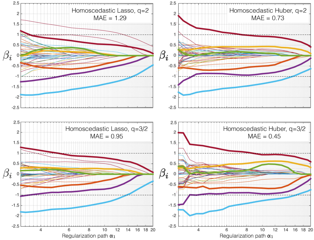
Figure 3: Generalized homoscedastic lasso and Huber solutions for b when q = 2 (top panel) and q = 3/2 (bottom panel) across the relevant \alpha_1 -path. The minimally achievable mean absolute error (MAE) is shown for all models. The six highlighted \beta_i trajectories mark the true non-zeros entries of \bar{b} . The dashed black lines show the values of the true \bar{b} entries.
