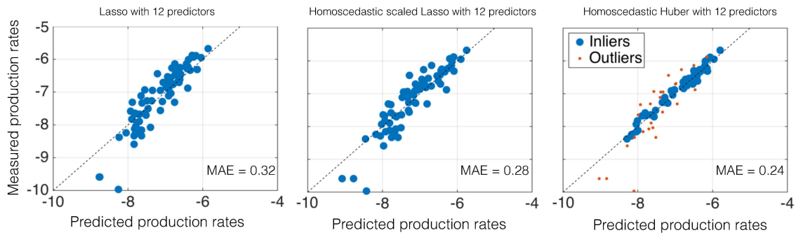
Figure 5: Standard lasso, homoscedastic lasso, and homoscedastic Huber log-production rate predictions with identical model complexity (every vector b comprises twelve non-zero components) and associated MAE (computed across all samples). The Huber M-estimator identifies 26 outliers (marked in red).
