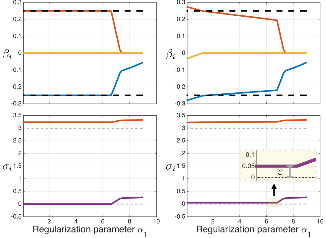
Figure 2: Generalized heteroscedastic lasso solutions for b (top panel) and s (bottom panel) across the \alpha_1 -path. The left panels show the results of fully non-smooth perspective M-estimation. The right panels show the results for a smoothed version with \sigma_i \in [\epsilon, +\infty[ for \epsilon = 0.05 . The dashed lines mark the ground truth entries of \bar{b} and \bar{s} .
